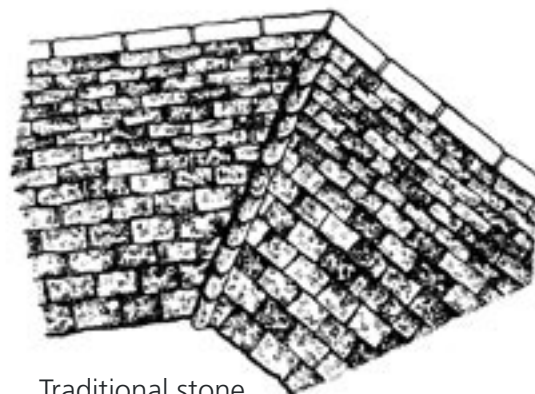
Traditional stone valley detail showing pointed valley slates
